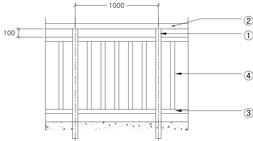
DETAIL SCALE : NONE
