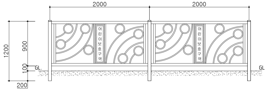
ELEVATION SCALE : NONE
