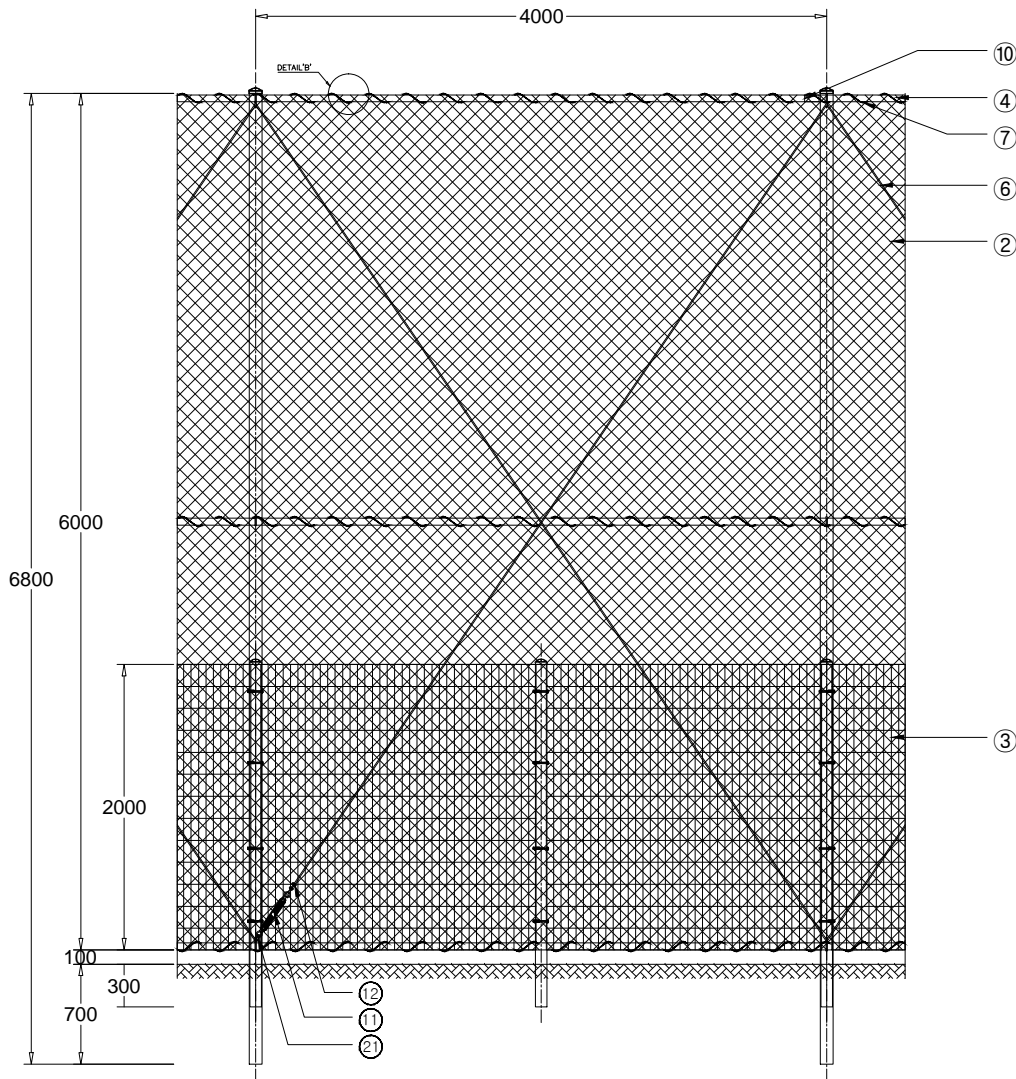
ELEVATION SCALE : NONE
