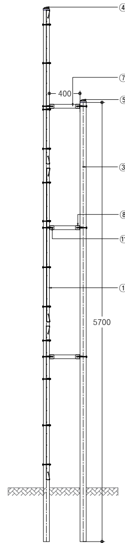
SIDE ELEVATION SCALE : NONE
