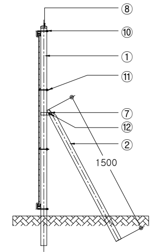
SIDE ELEVATION SCALE : NONE
