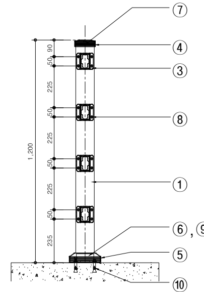
SIDE ELEVATION SCALE : NONE
